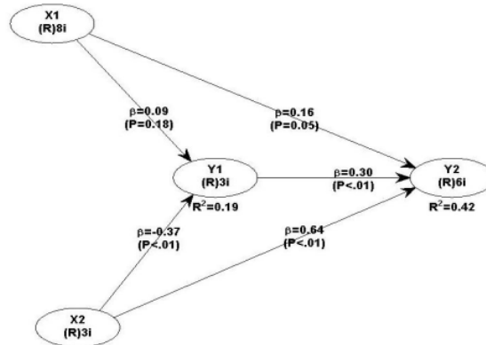
Gambar 1. Structural Equation Modeling
